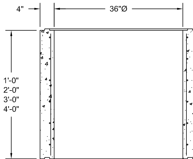
Standard Available Extensions
