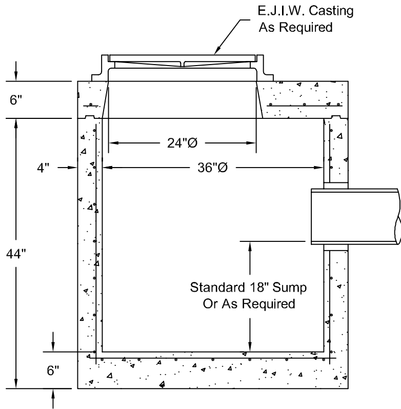
Standard Bottom Section w/ Integral Base
