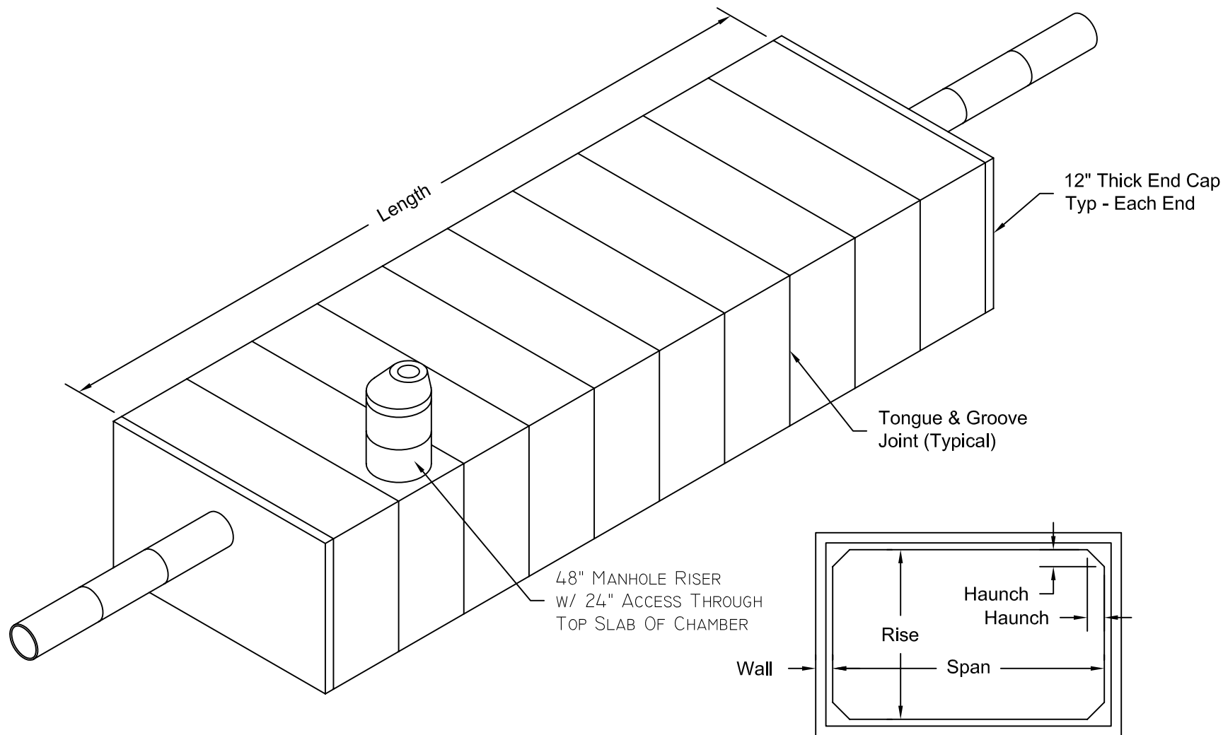
For Spans 24'-0" Or Less
