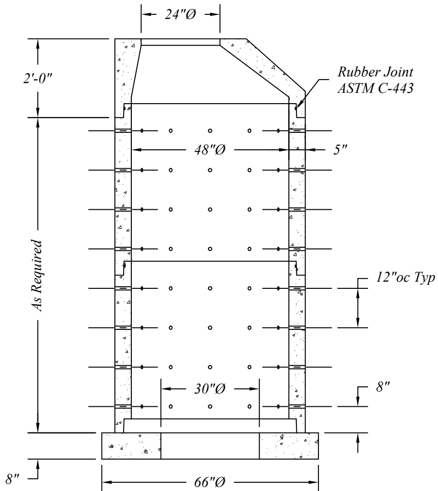
Typical 48"Ø Precast Concrete Leach Basin
