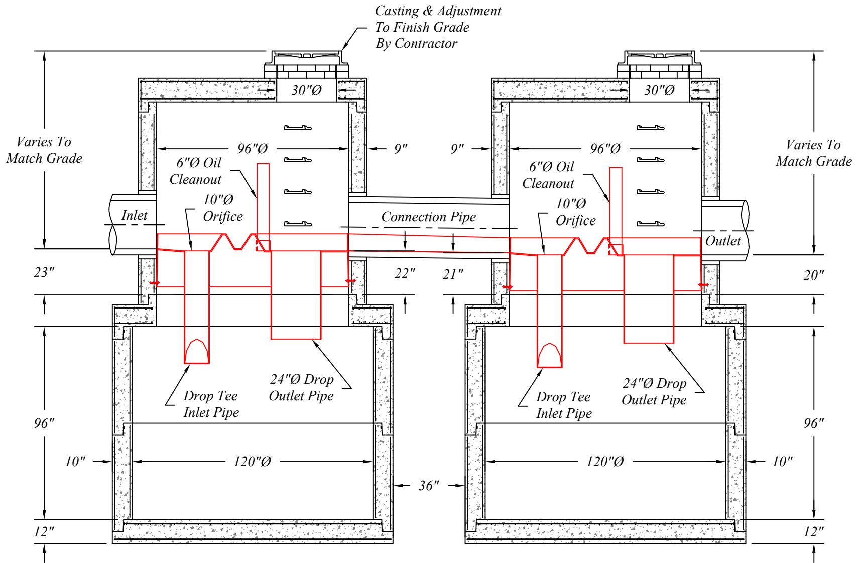
Section Thru Chambers
