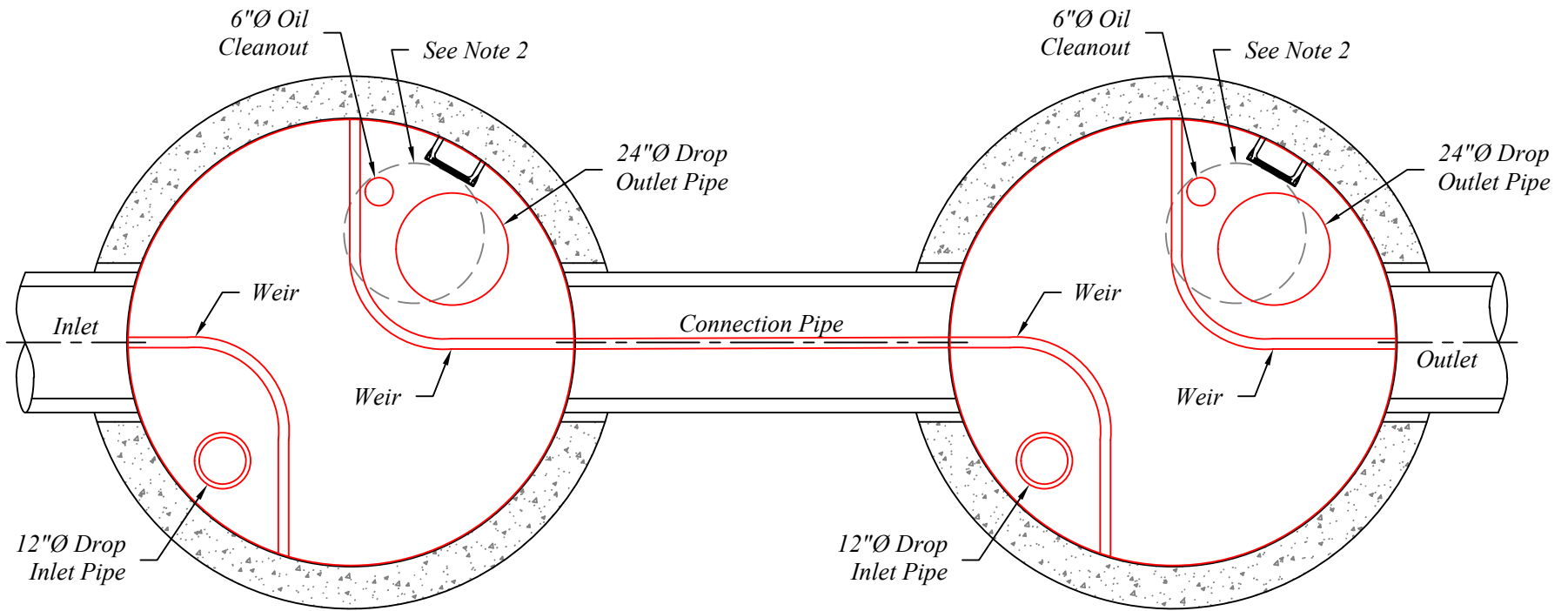
Plan View
