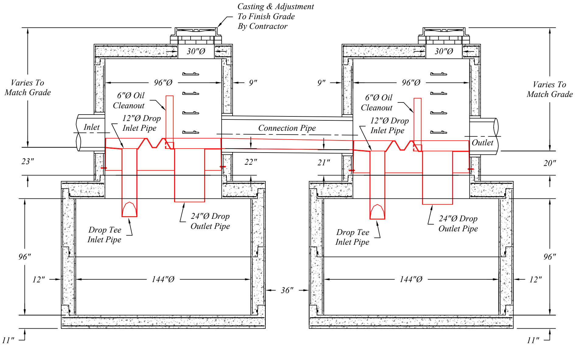
Section Thru Chambers
