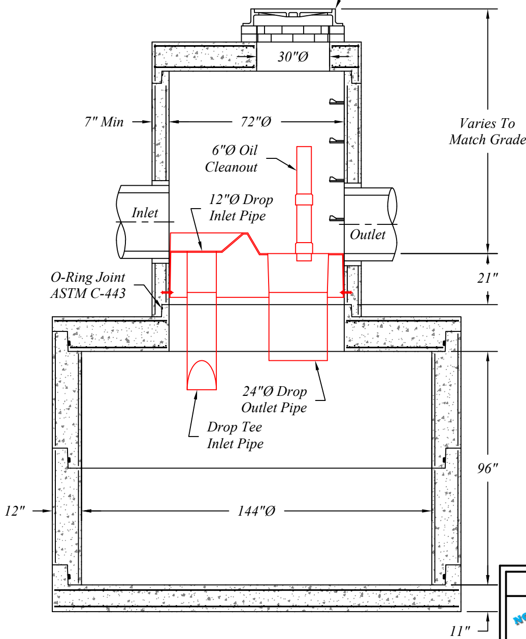
Section Thru Chamber
